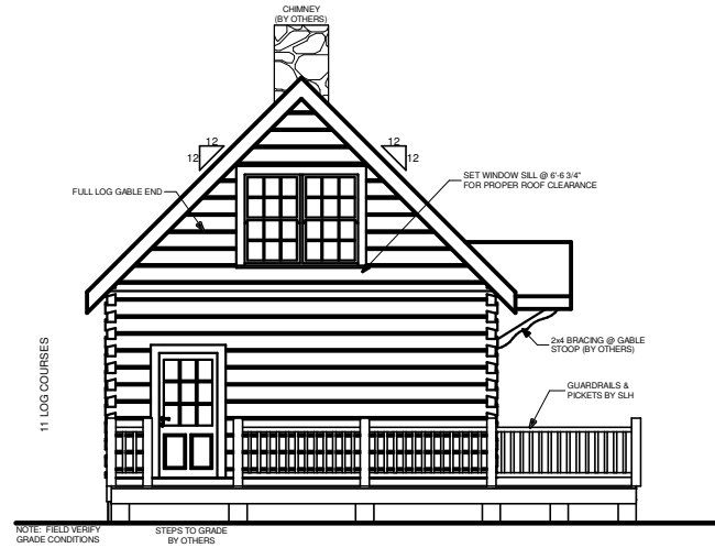
LEFT ELEVATION
