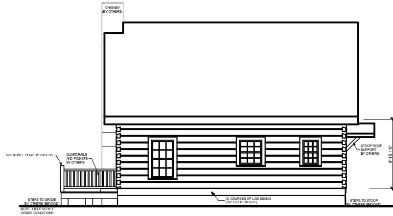
REAR ELEVATION
