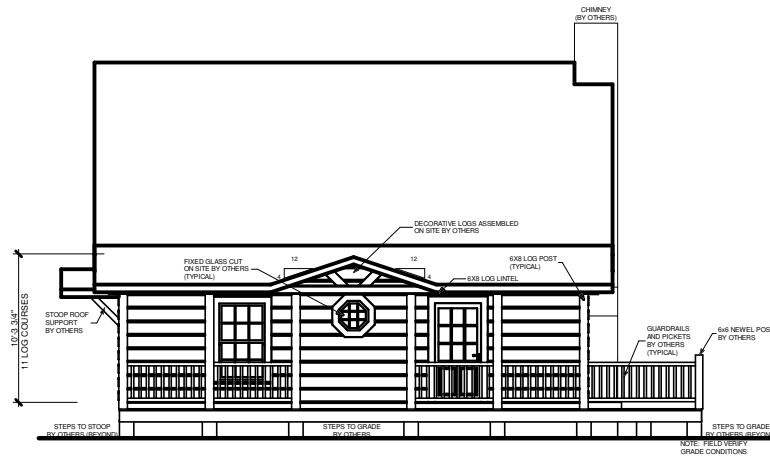
FRONT ELEVATION 14'x11'0"
