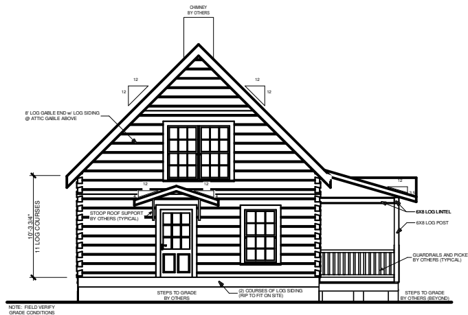
LEFT ELEVATION
