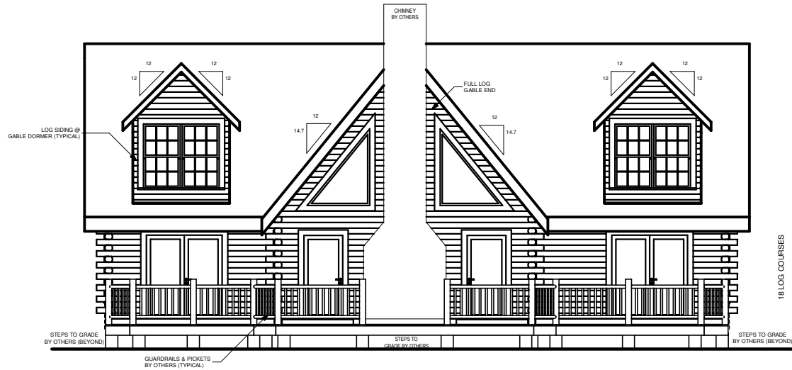
REAR ELEVATION
