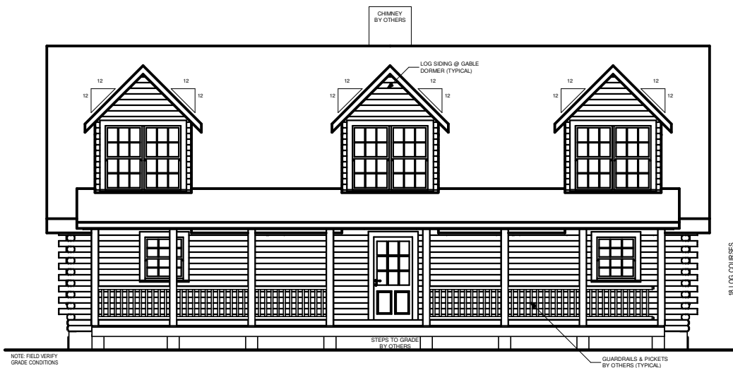
FRONT ELEVATION
