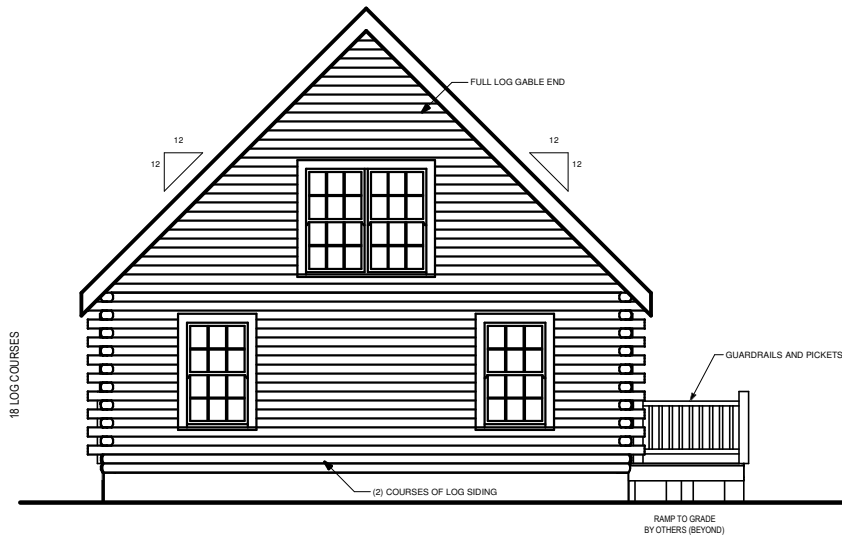
REAR ELEVATION
