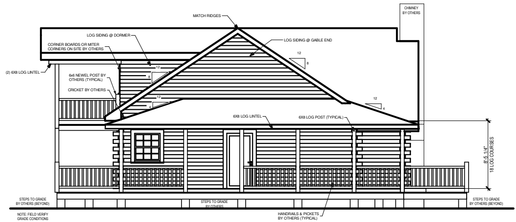
LEFT ELEVATION
