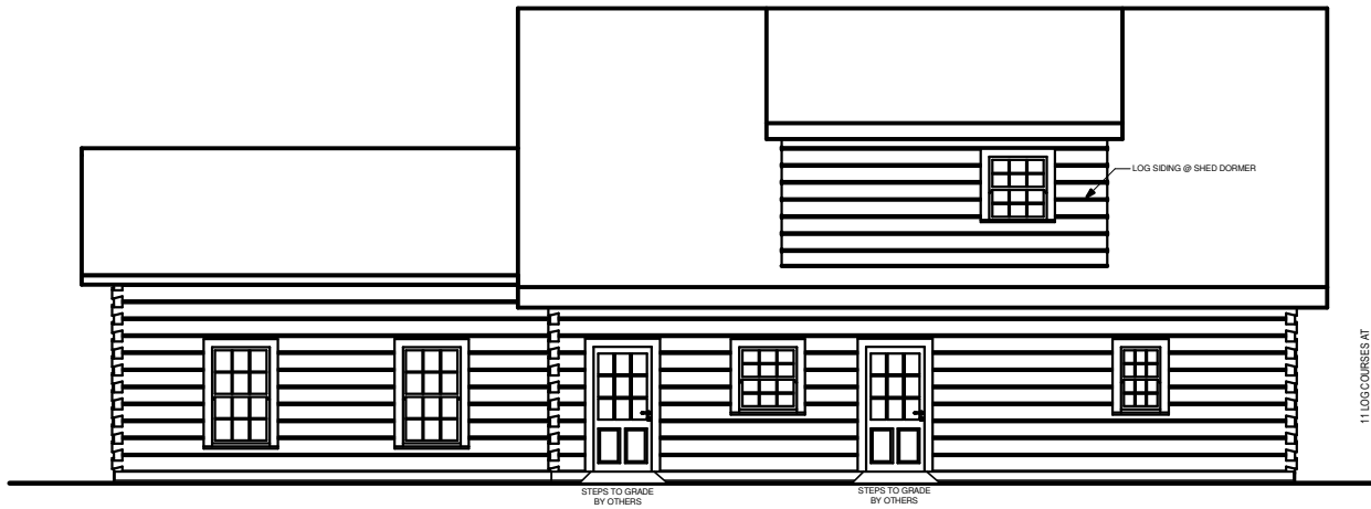
REAR ELEVATION
