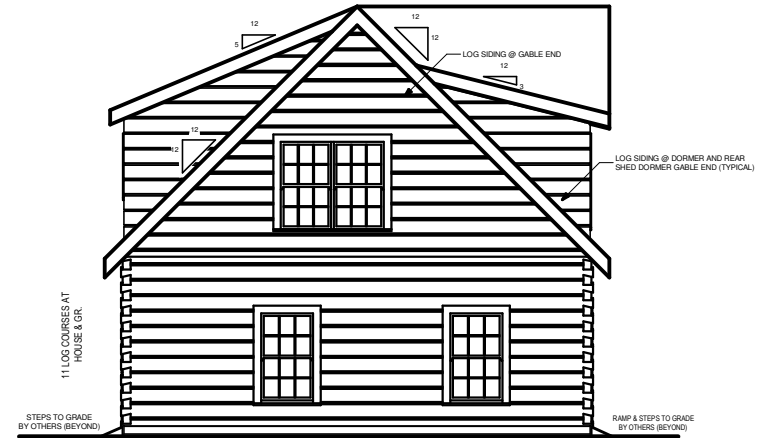
LEFT ELEVATION
