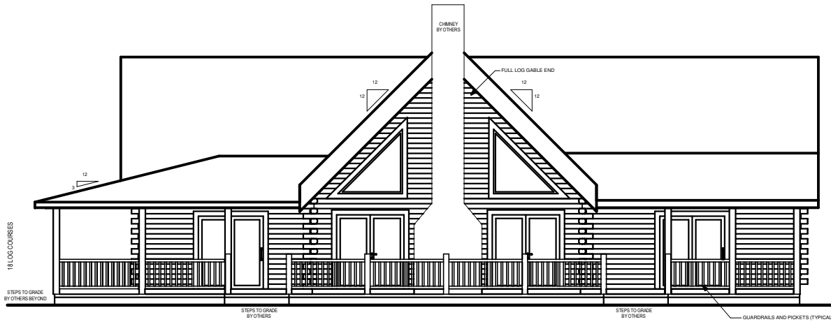
FRONT ELEVATION
