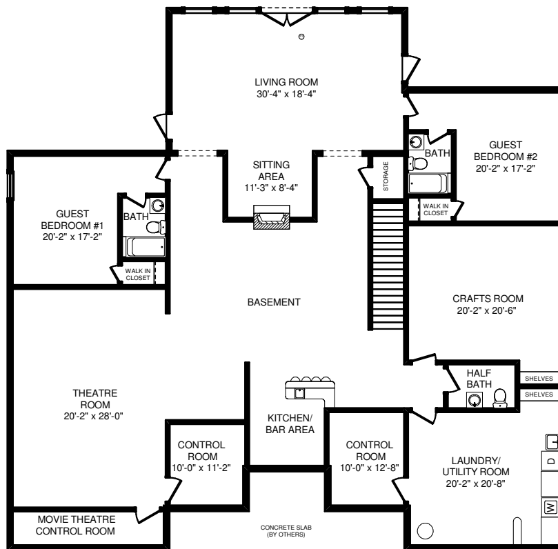
BASEMENT PLAN
