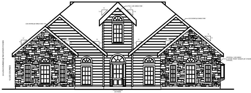
FRONT ELEVATION
