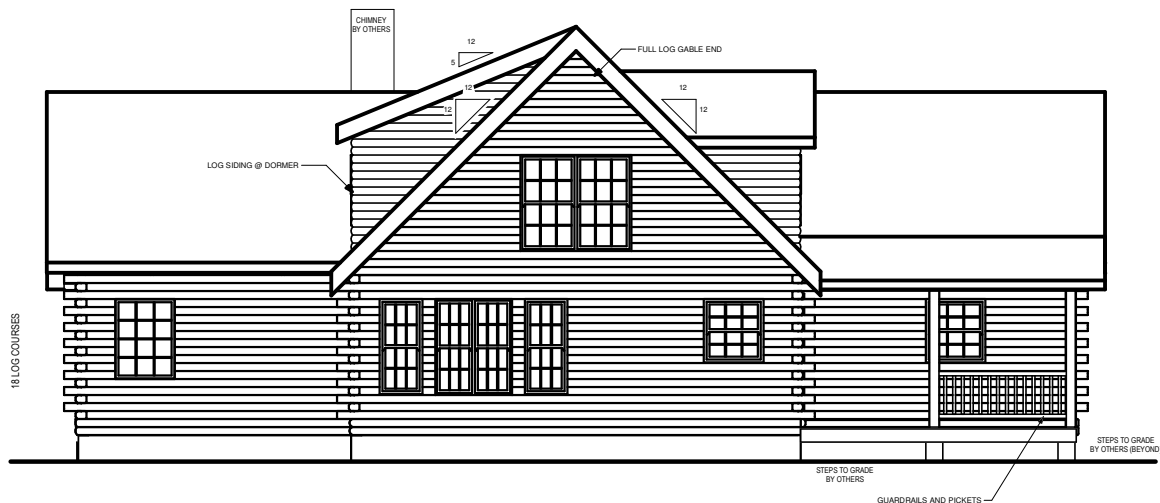
REAR ELEVATION
