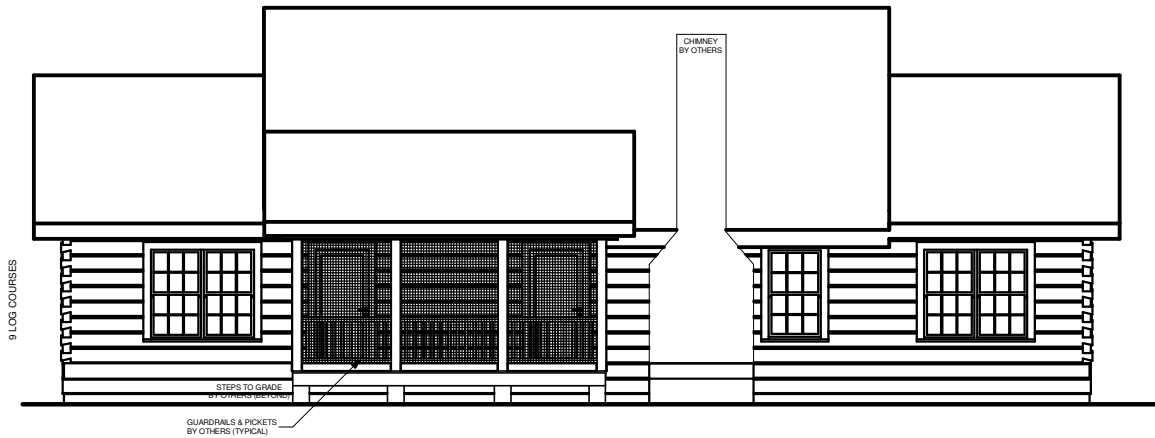
REAR ELEVATION
