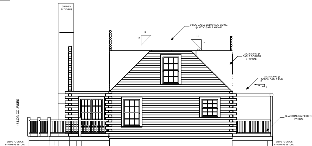
LEFT ELEVATION
