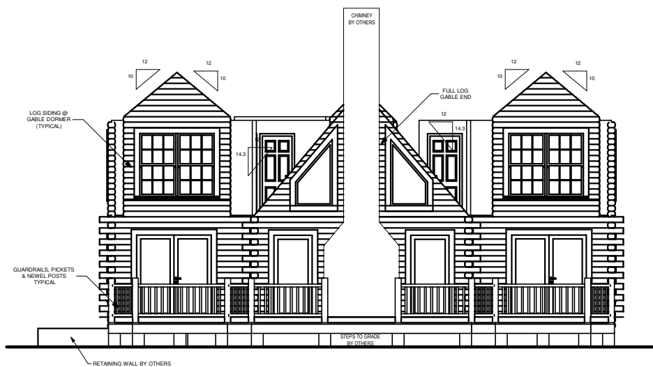
REAR ELEVATION
