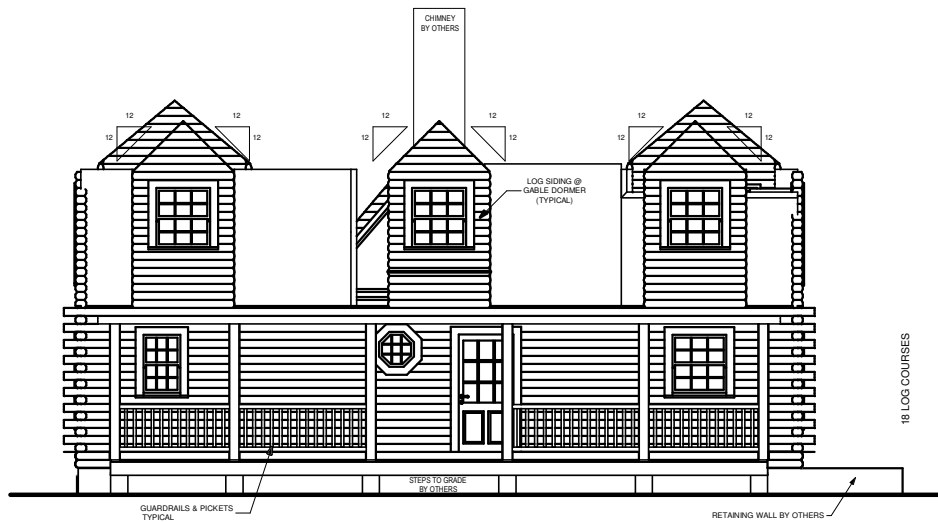
FRONT ELEVATION
