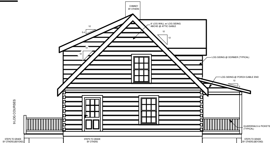
LEFT ELEVATION
