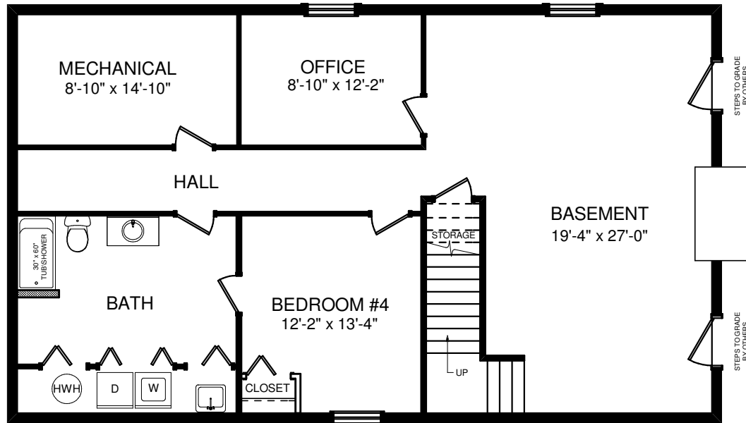
BASEMENT PLAN
