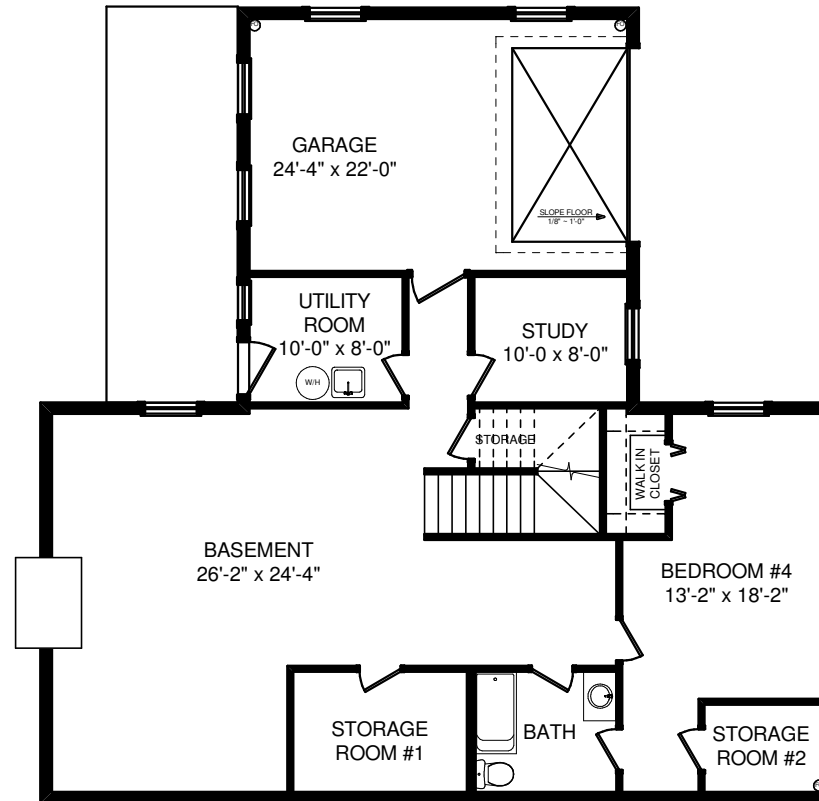
BASEMENT PLAN
