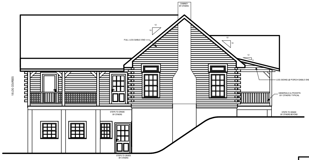
LEFT ELEVATION
