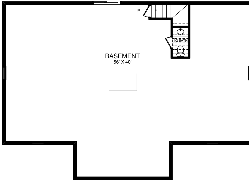
BASEMENT PLAN
