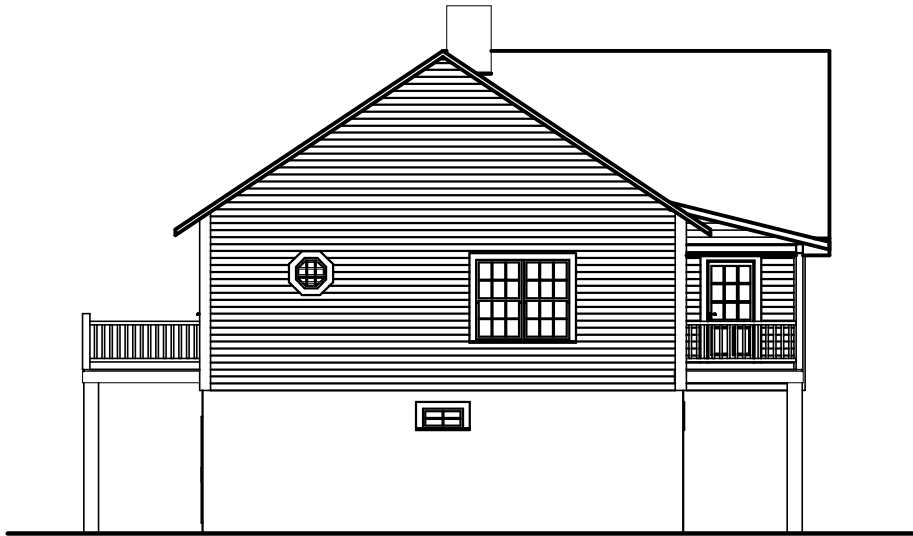
LEFT ELEVATION
