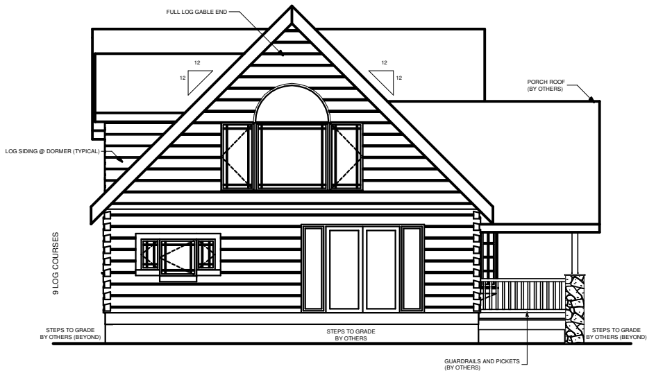
LEFT ELEVATION
