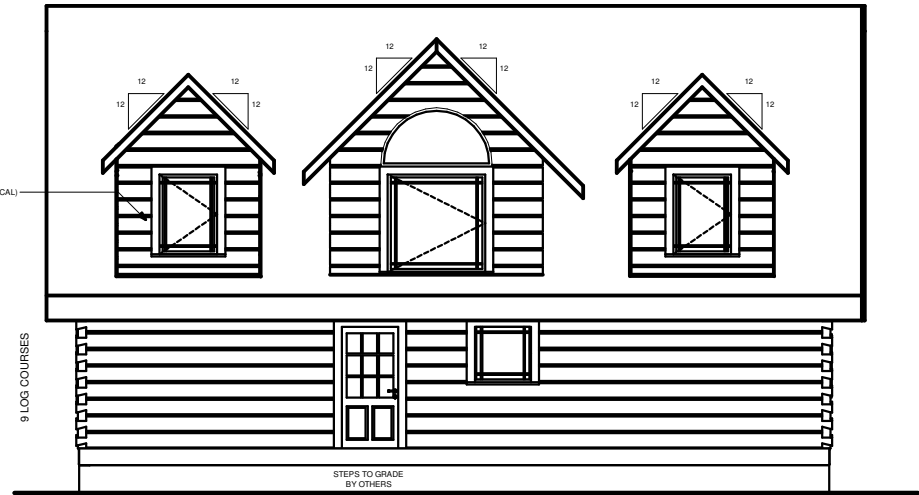
REAR ELEVATION
