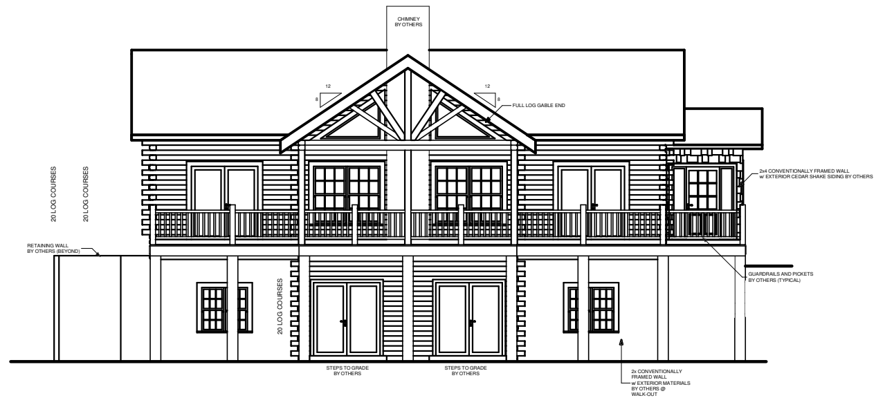
FRONT ELEVATION
