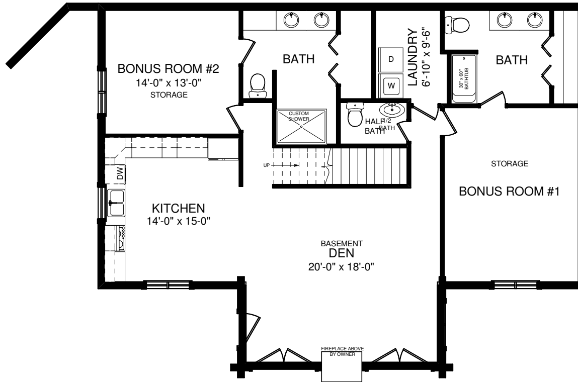
BASEMENT PLAN
