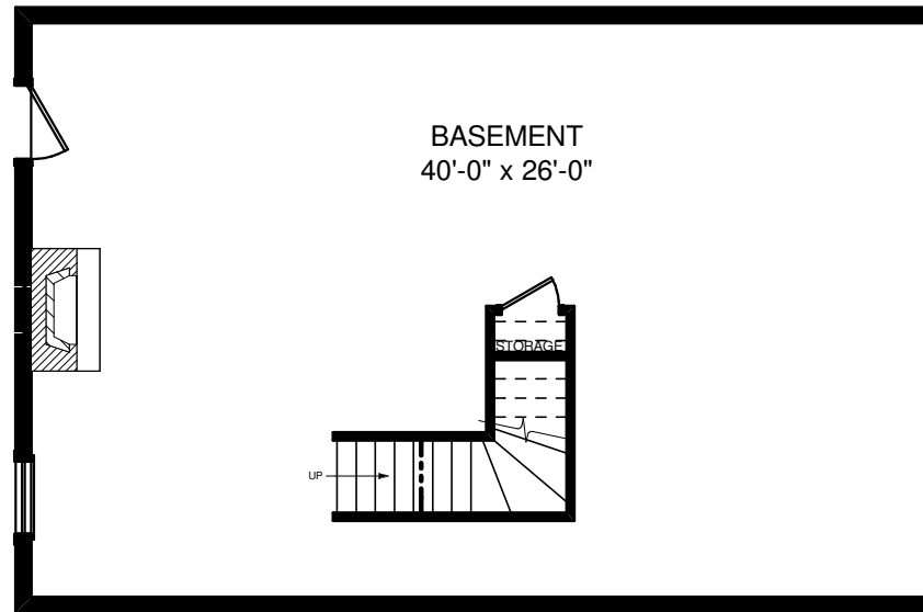
BASEMENT PLAN
