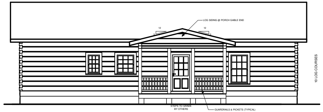
FRONT ELEVATION
