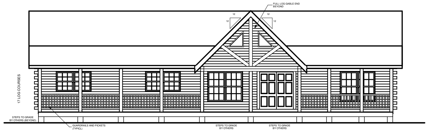
FRONT ELEVATION
