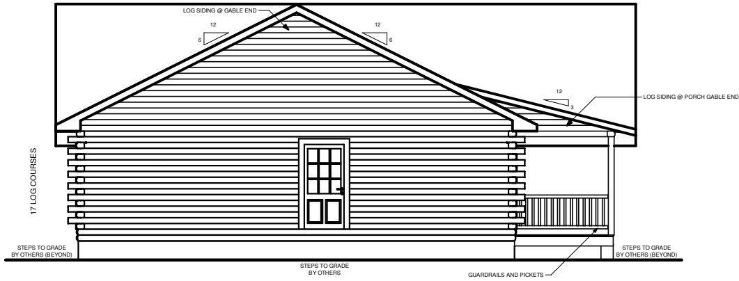
LEFT ELEVATION
