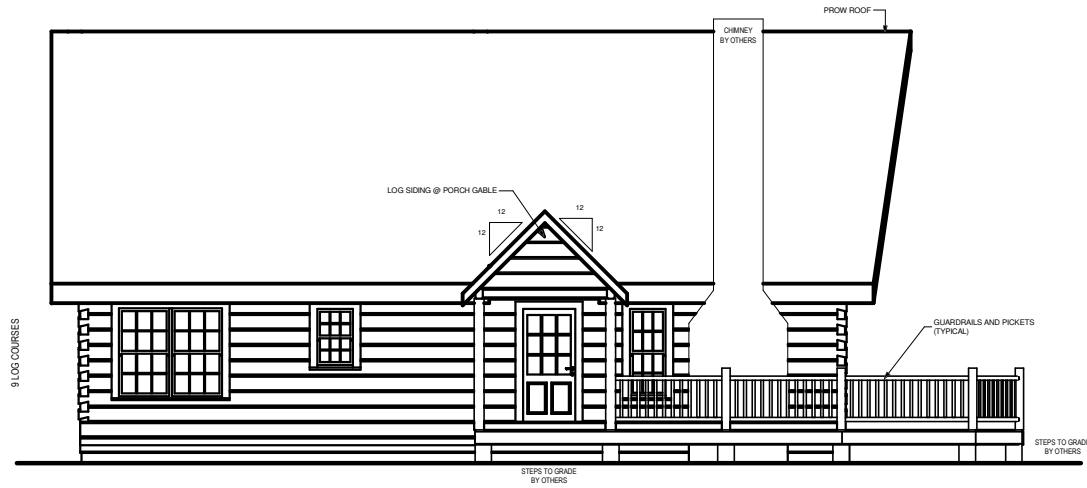
LEFT ELEVATION
