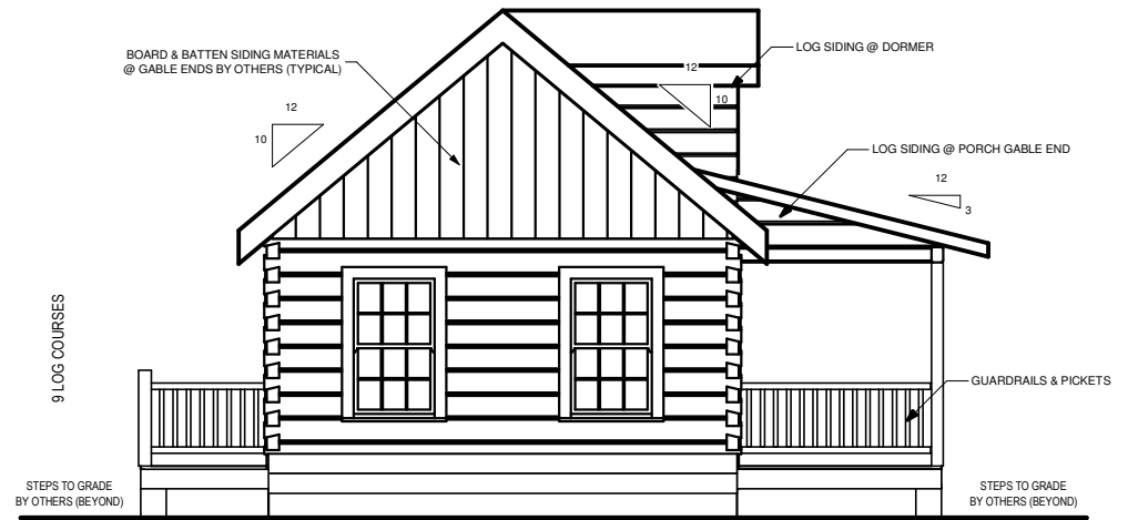
LEFT ELEVATION
