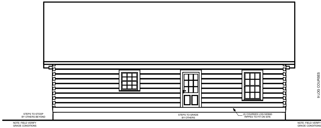
REAR ELEVATION
