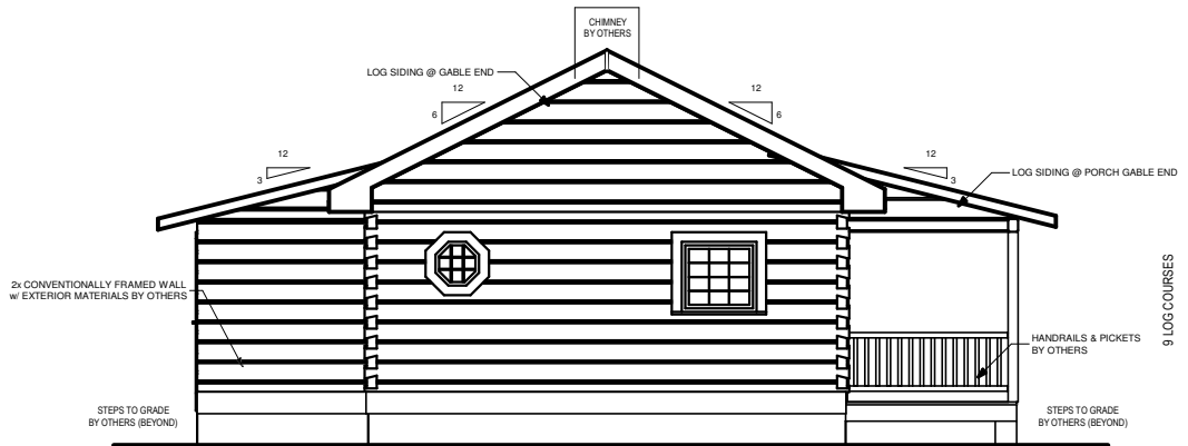
LEFT ELEVATION
