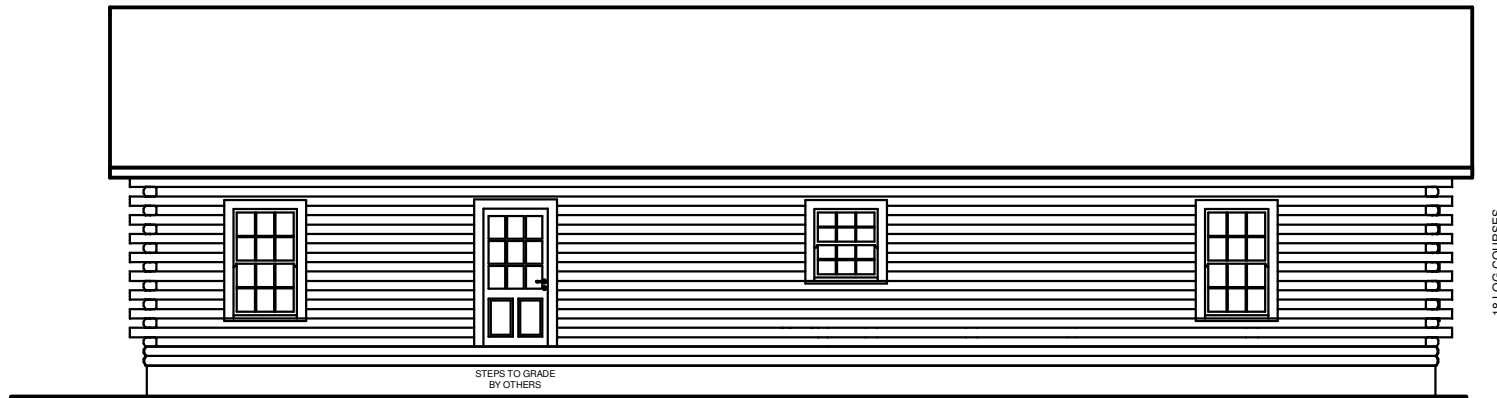
REAR ELEVATION
