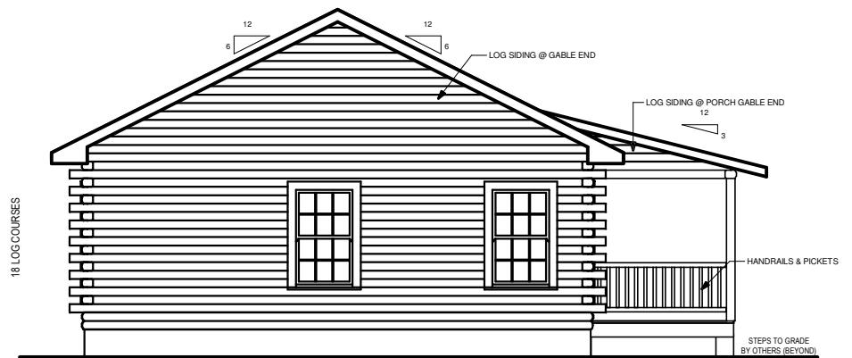
LEFT ELEVATION
