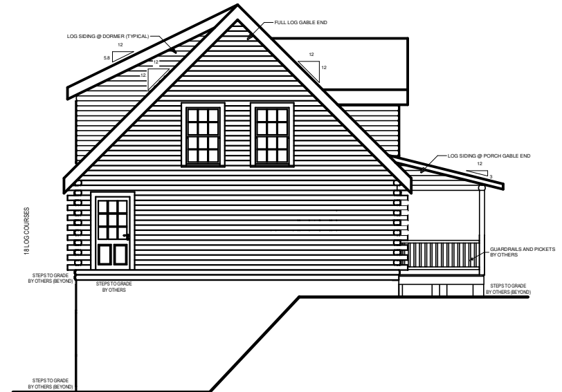
LEFT ELEVATION
