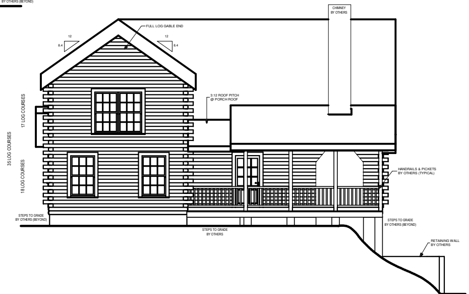
LEFT ELEVATION
