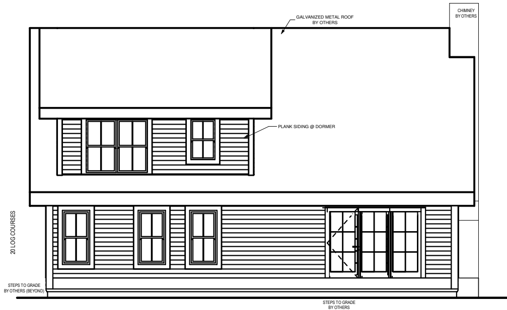
REAR ELEVATION
