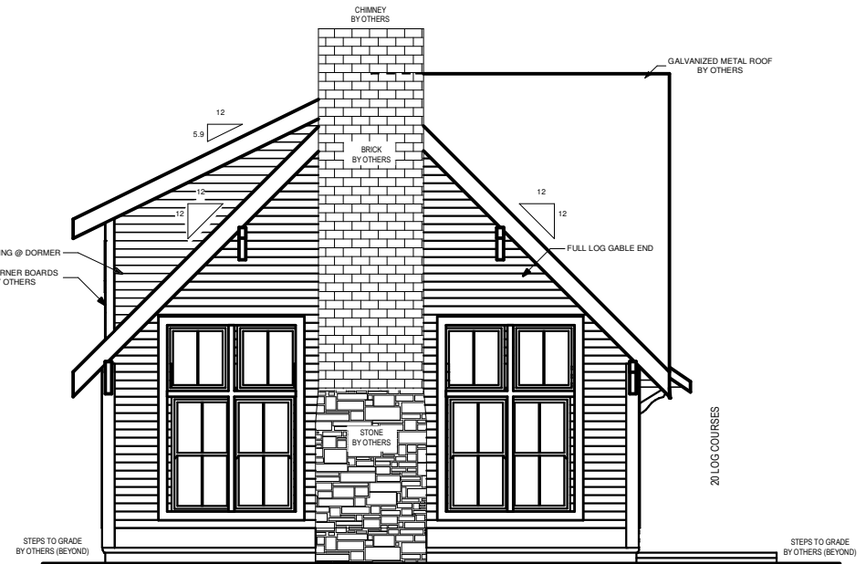
LEFT ELEVATION
