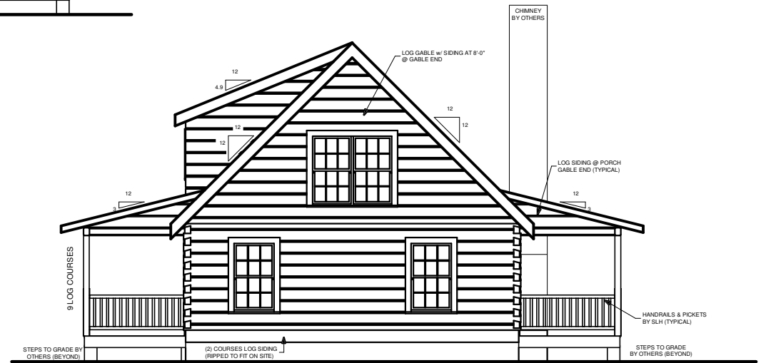
LEFT ELEVATION
