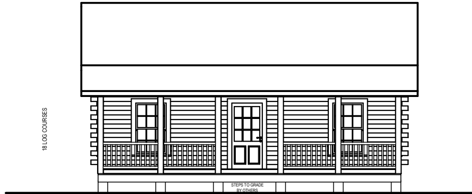
LEFT ELEVATION
